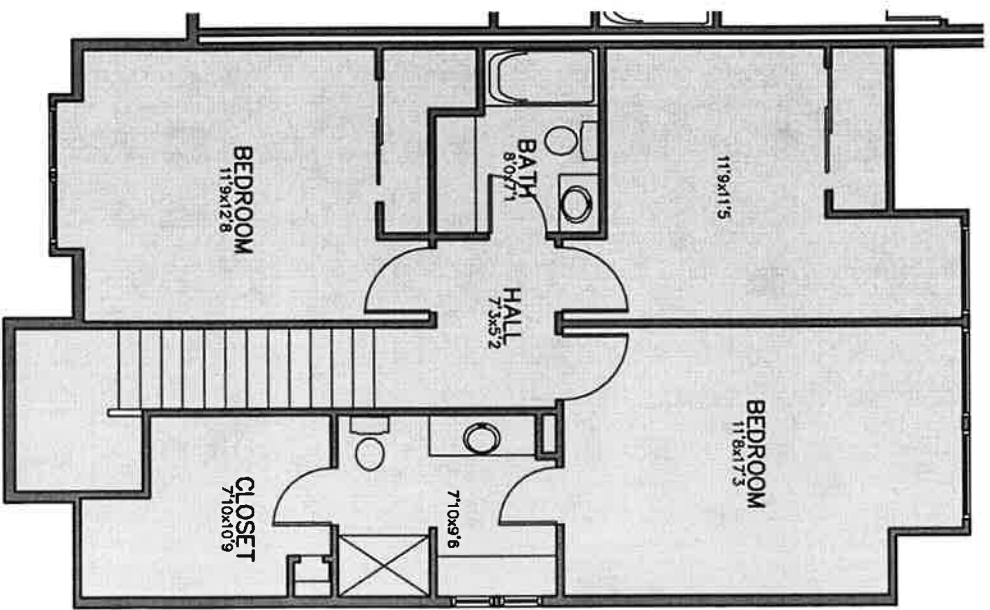
2 UNIT B SECOND FLOOR PLAN SCALE: 1/8" = 1'-0" 0 2' 4' 6'
