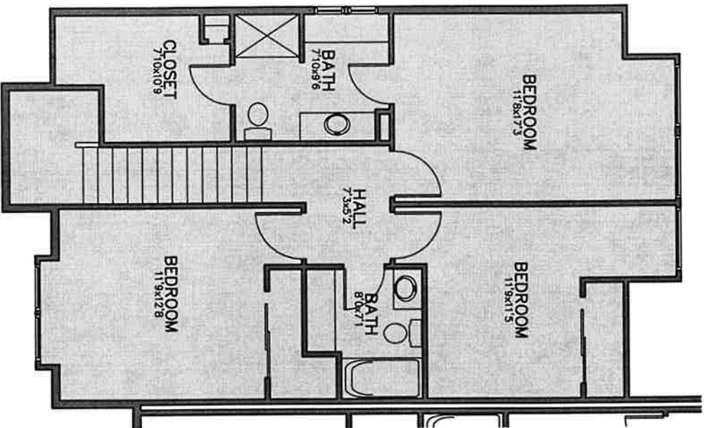
2 UNIT C SECOND FLOOR PLAN SCALE: 1/8" = 1'-0" 0 2' 4' 6'
