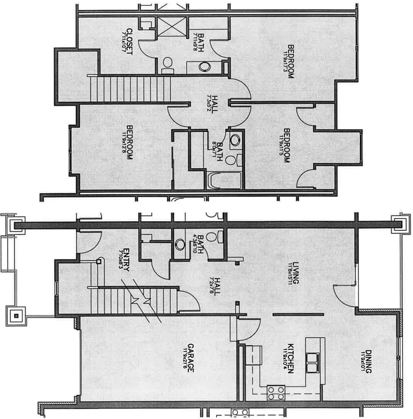
2 UNIT A SECOND FLOOR PLAN A1.2
