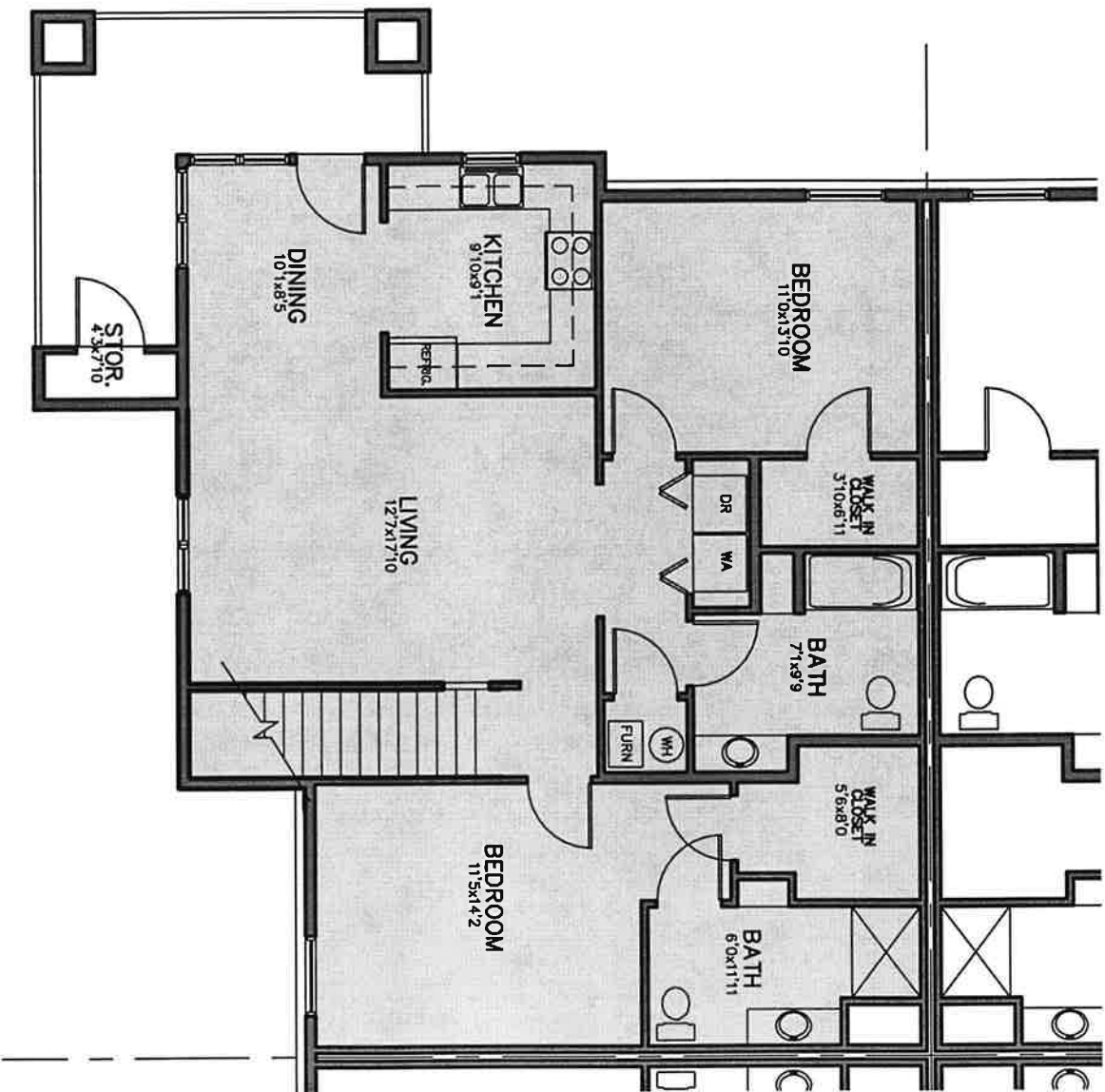
1 A2 TYPICAL UPPER PLAN SCALE: 1/8" = 1'-0"
